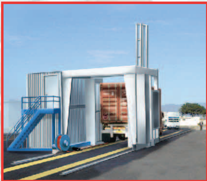
Shaped Energy™ 3.5 MeV Gantry configuration, Densely packed container inspection
